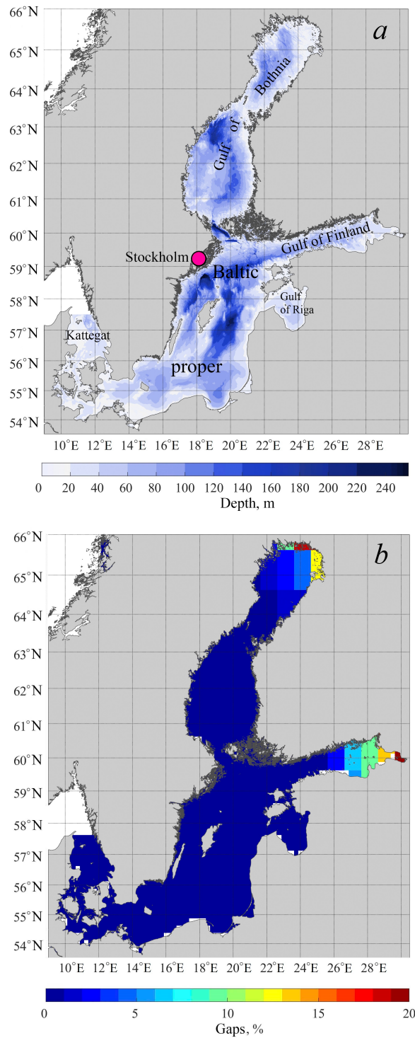
Fig. 1. Bathymetry map of the Baltic Sea and location of the Stockholm tide gauge station (a), number of gaps (as a percentage of the total number of series terms) in the nodes of altimetry data grid area (b)
