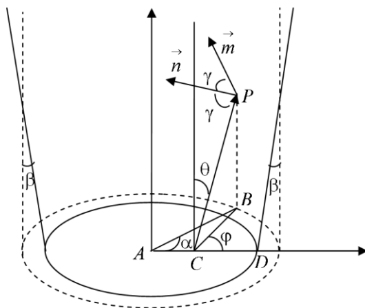
Fig. 3. Scheme of a scattered beam propagation in a cone cuvette used for calculating a path length, reflection angles and their number
