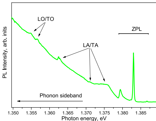
Fig. 3. Fine structure of the emission spectrum for crystal ZnSe:Fe in the zero-phonon line (ZPL) transition region {}^3T_1({}^3H) \rightarrow {}^5E({}^5D) at a temperature of 5K. For PL excitation, radiation with a wavelength of 532 nm is used. LO/TO and LA/TA denote phonon replicas involving optical and acoustic phonons, respectively
